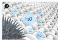
OH radicals transform hydrogen to inhibit the activity of pollutants
