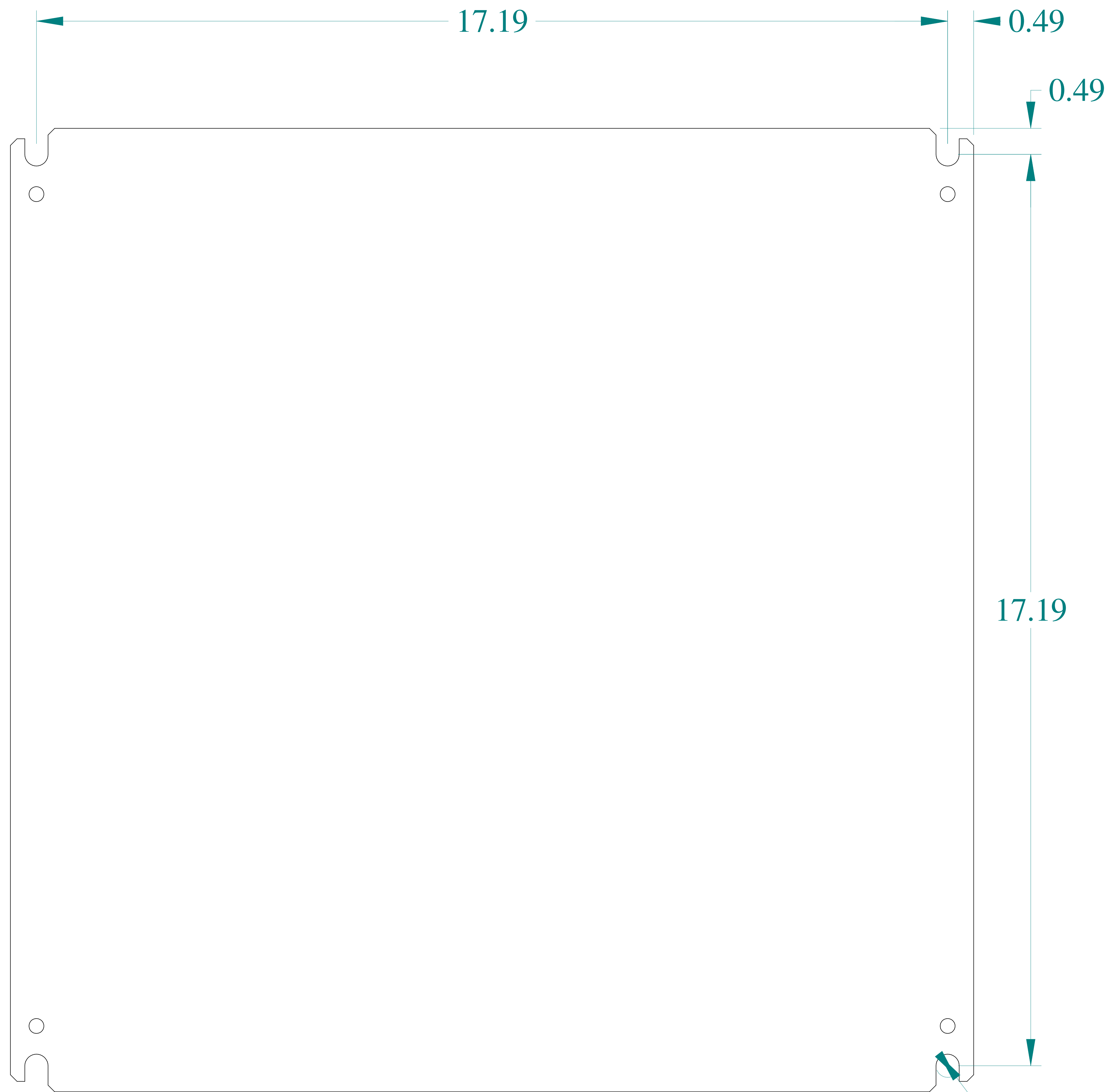
FRONT VIEW
