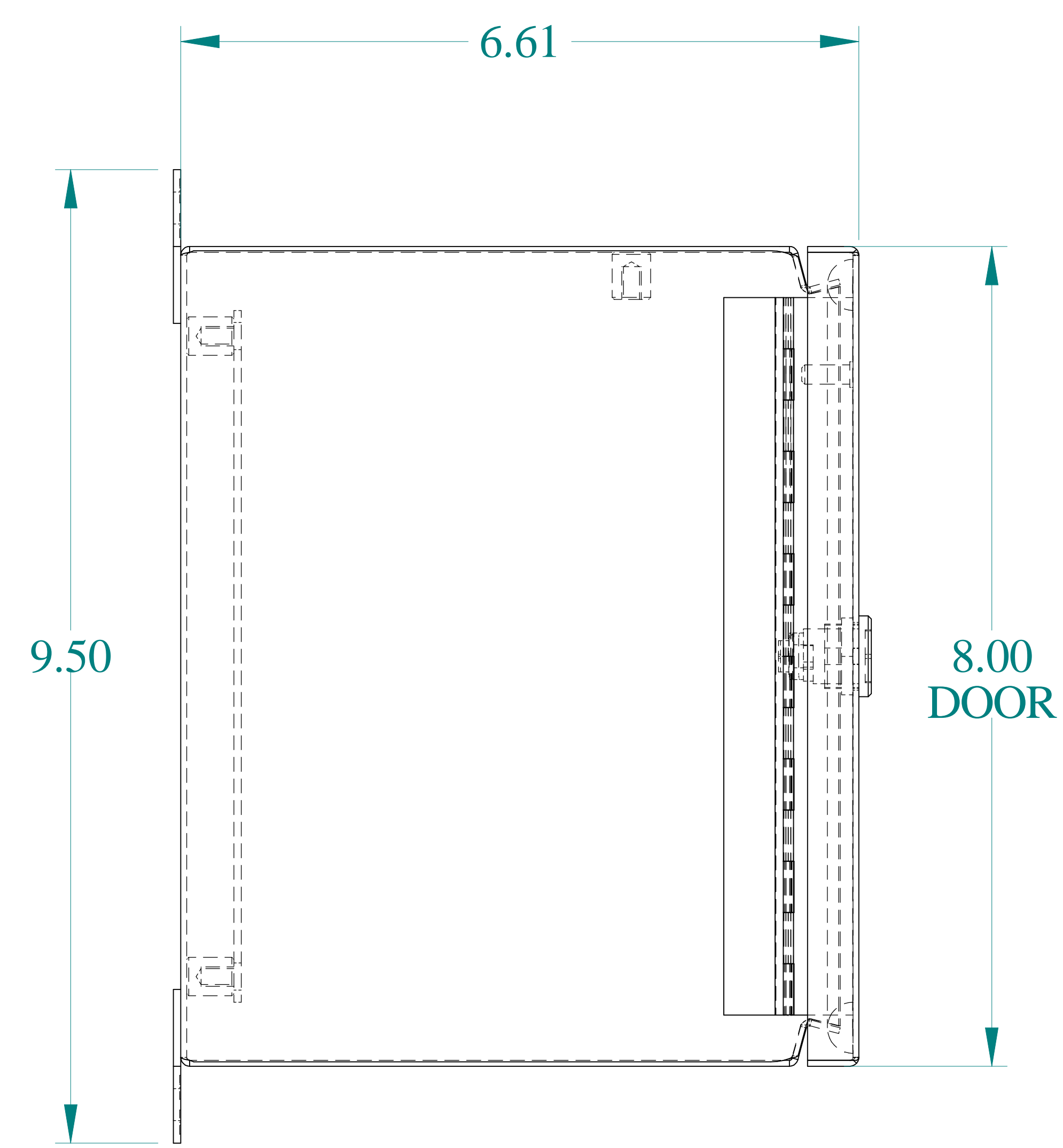
SIDE VIEW
