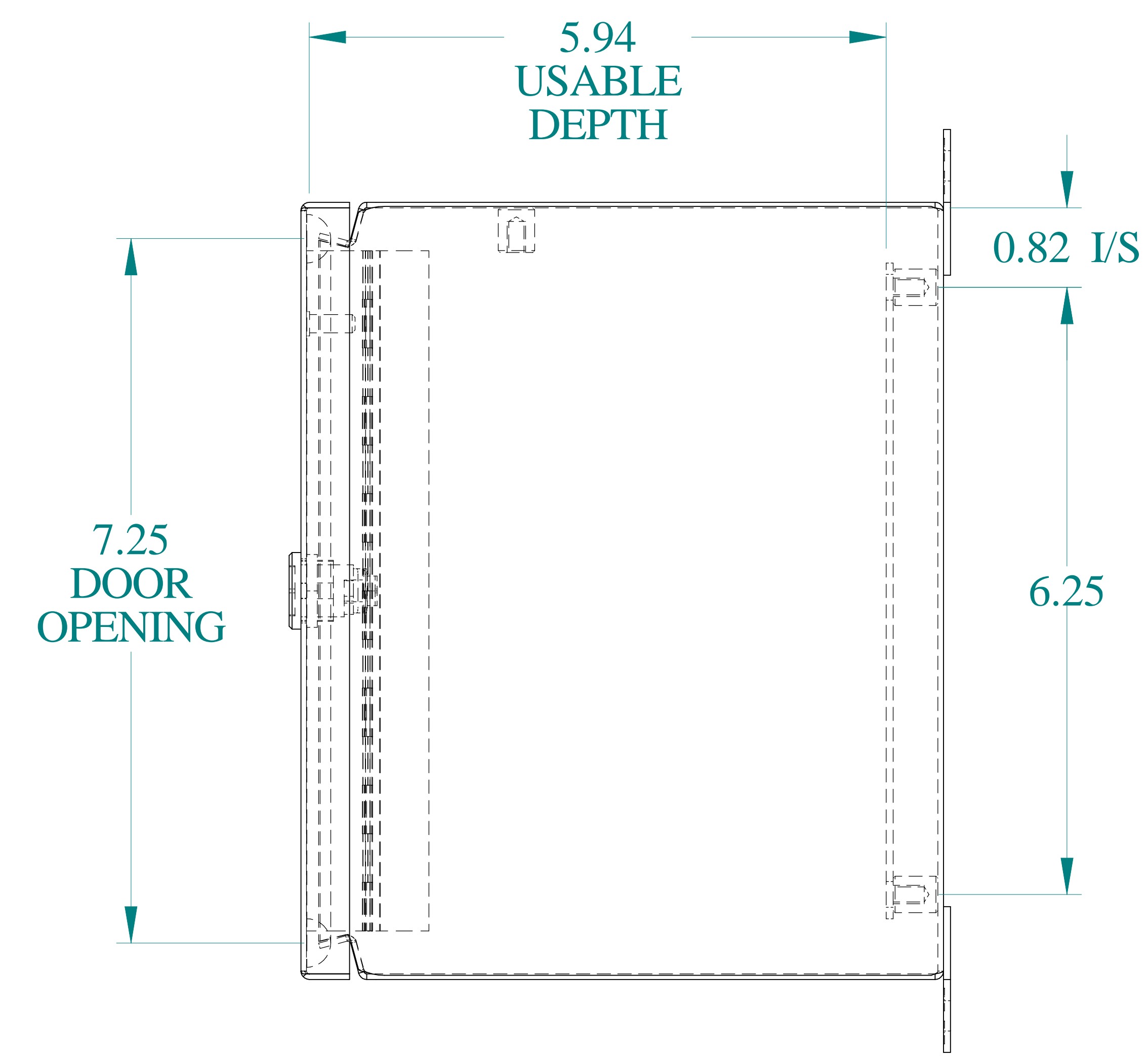
SIDE VIEW
