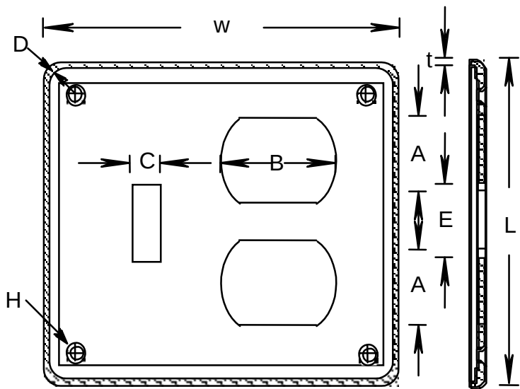
COMBO SWITCH RECEPTACLE, TYPE TSDC. 077739
