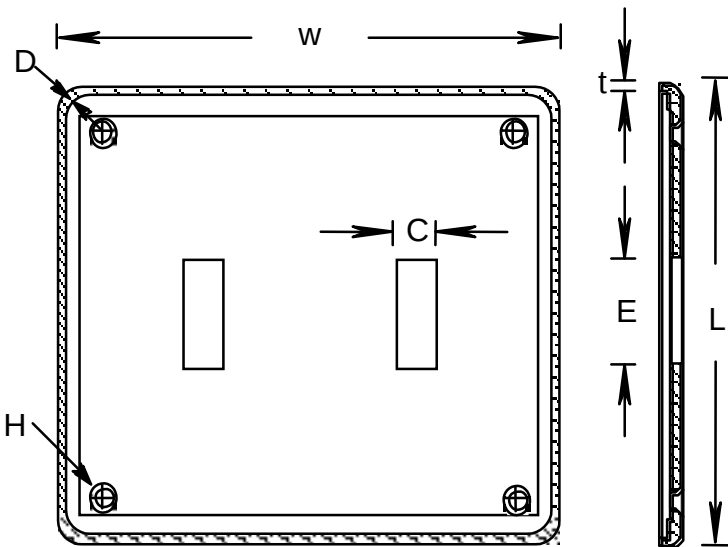
DOUBLE SWITCH, TYPE TSC, 077738
