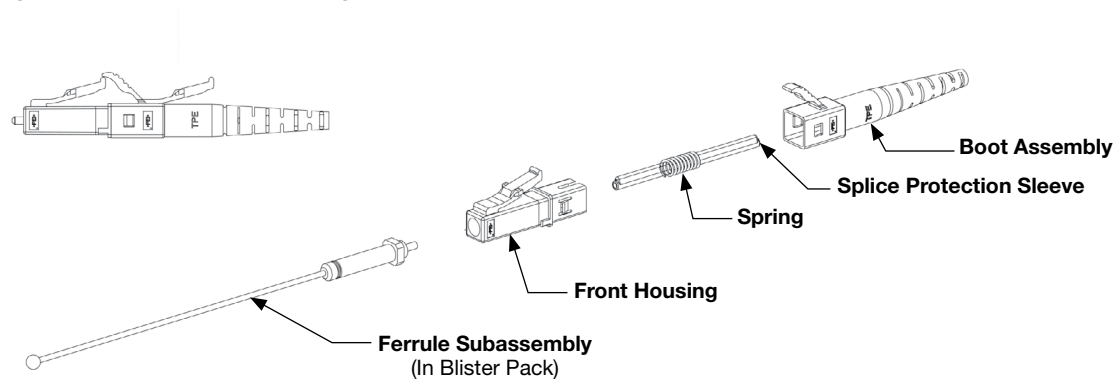
Fiber LC Splice-on Connector For 250/900µm Fiber
