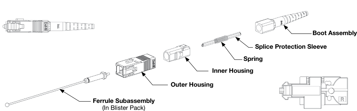
Fiber SC Splice-on Connector For 250/900µm Fiber
