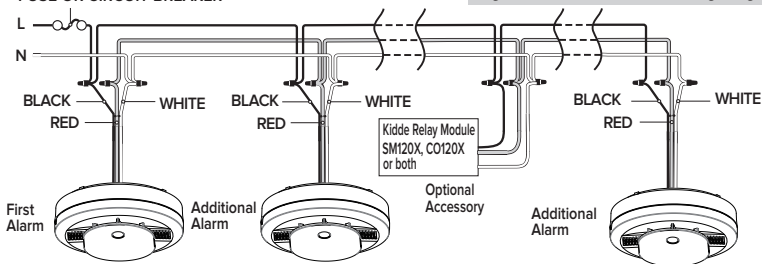
Figure 8-A, Interconnect Wiring Diagram
