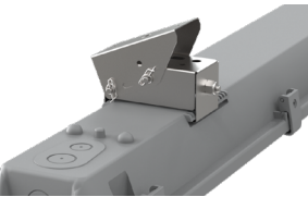
Shown with CSVTRMBA Bracket can be set to 22.5°, 45° or 90° angles.
