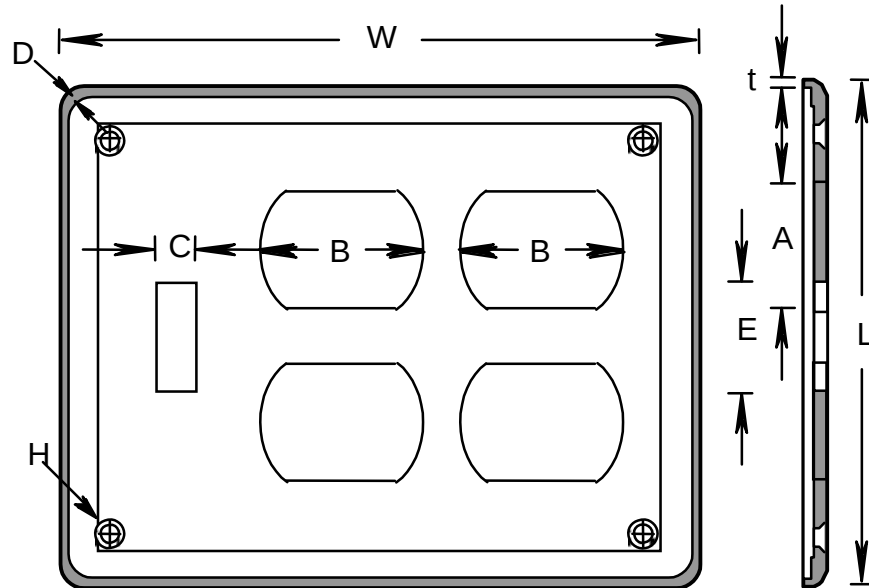
SINGLE SWITCH DOUBLE RECEPTACLE, TYPE TSDC20-3 CODE: 077746
