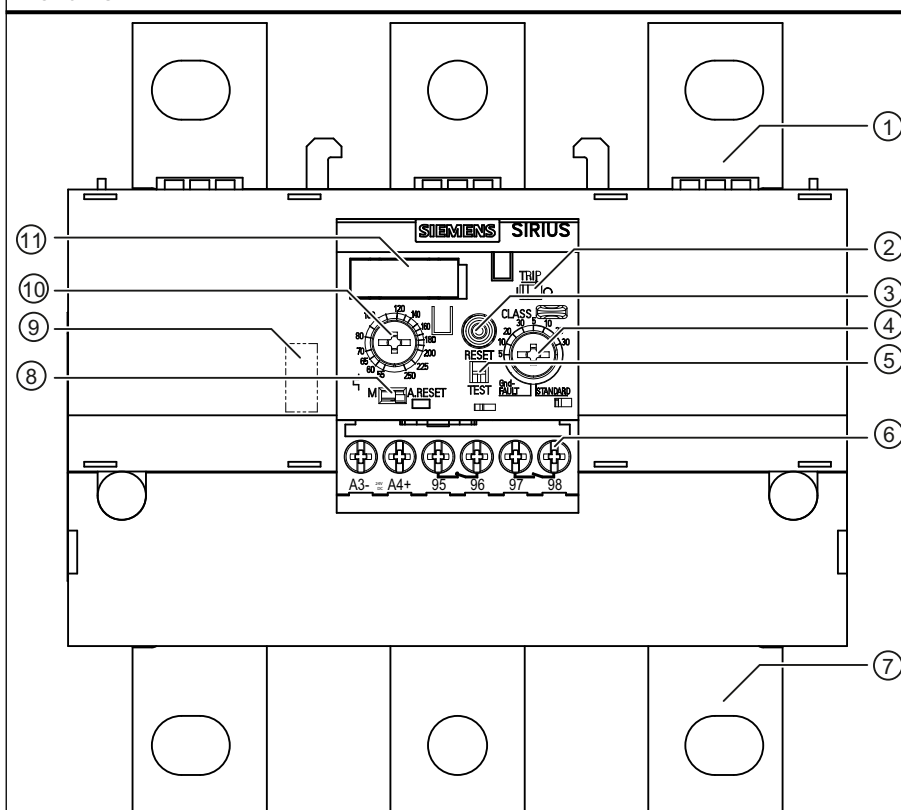
3RB2163 overload relay equipment
