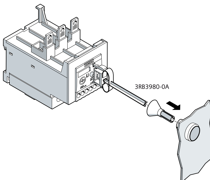
Mounting a mechanical remote RESET to a 3RB3.4 electronic overload relay.
