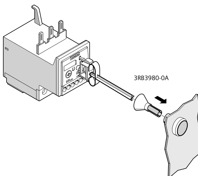
Mounting a mechanical remote RESET to a 3RB3.3 electronic overload relay.
