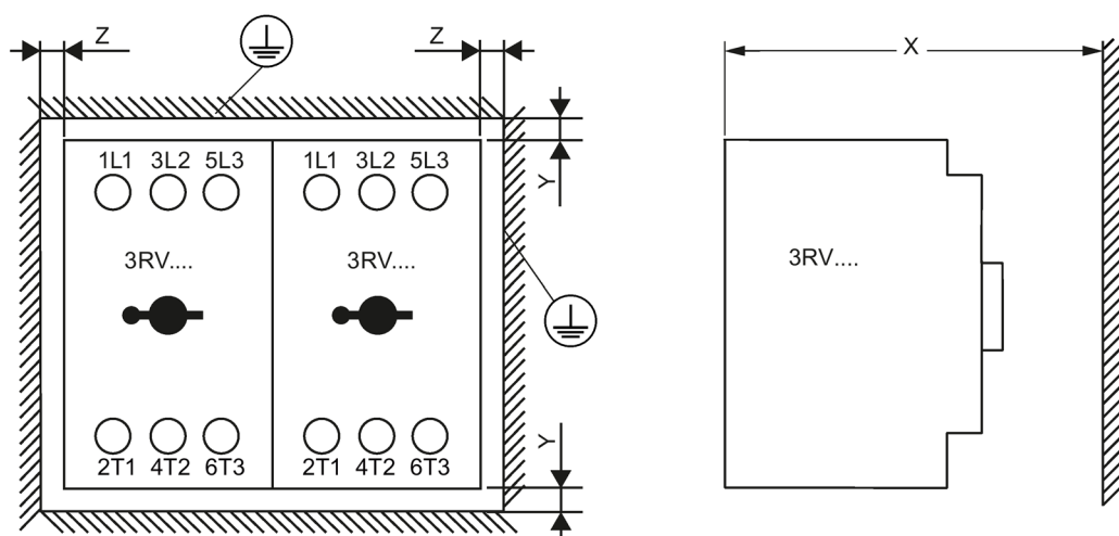
Figure 8-1 Clearances from grounded or live parts
