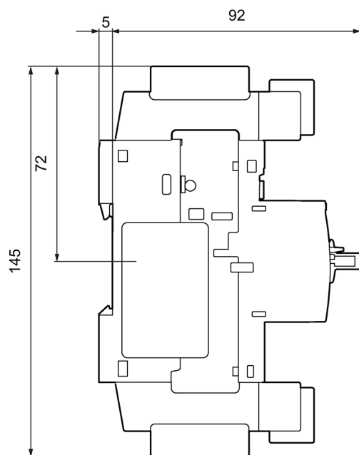
Figure C-8 Circuit breaker acc. to UL 489
