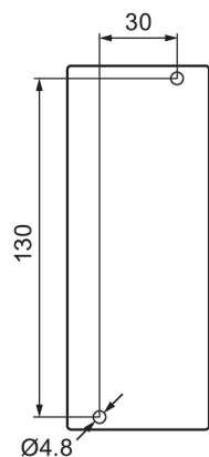
Figure C-12 3RV2.3 motor starter protector
