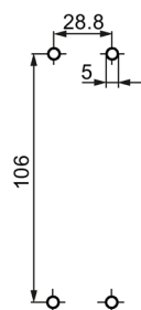
Figure C-9 Motor starter protectors S00 / S0 with lugs for screw fastening
