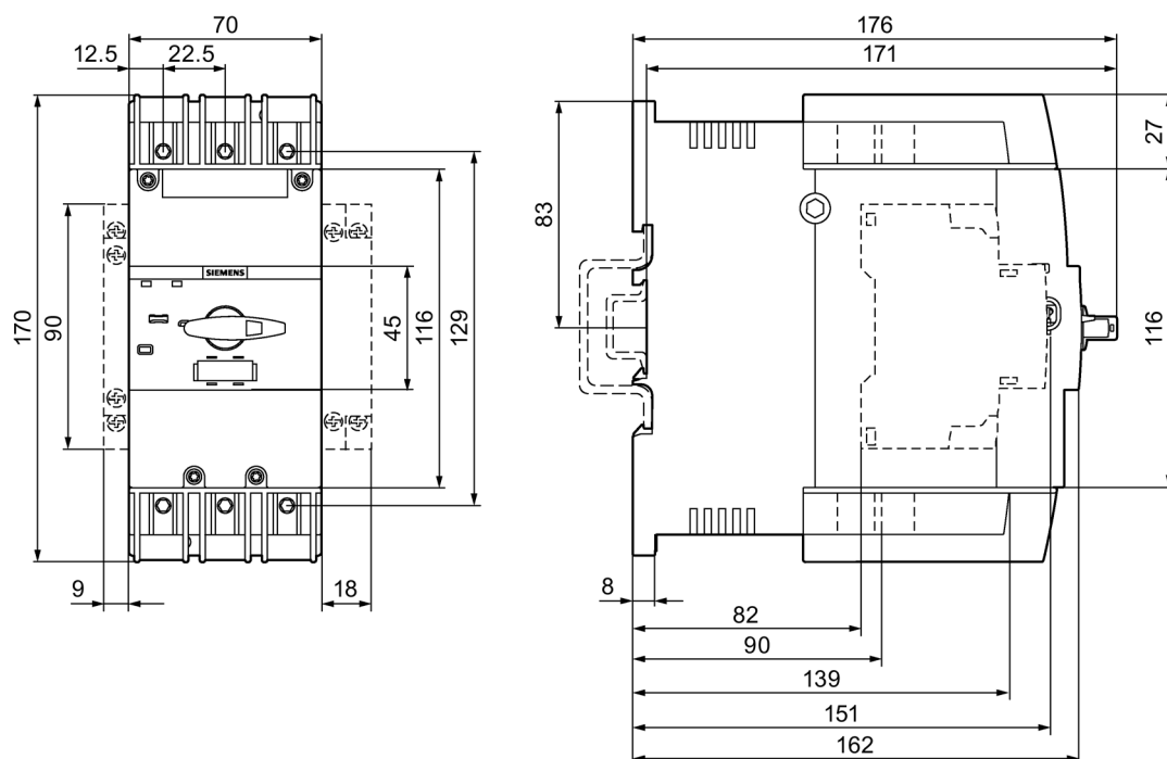
Figure C-14 Circuit breaker acc. to UL 489
