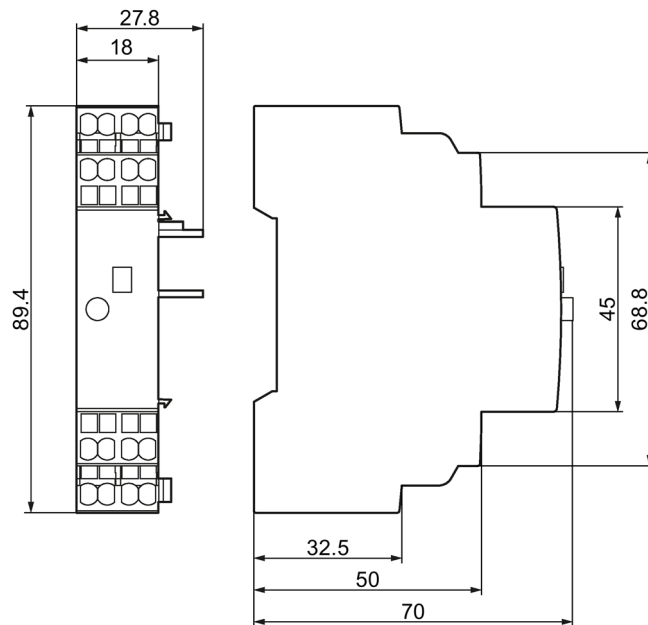
Figure C-45 3RV2921-2M signaling switch (spring-type connection)
