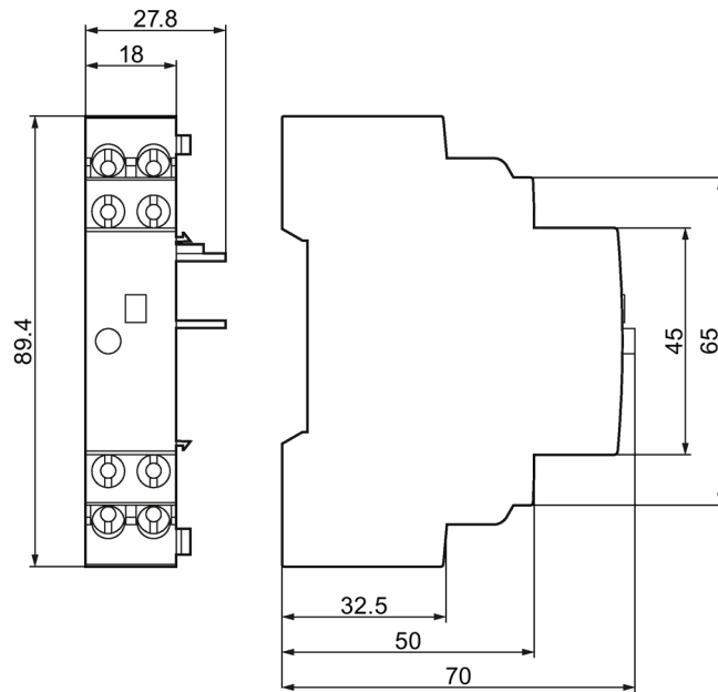
Figure C-44 3RV2921-1M signaling switch (screw-type connection system)
