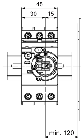
Figure C-30 3RV2.1 and 3RV2.2
