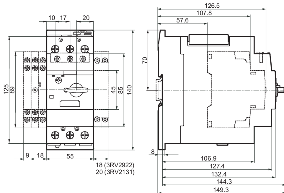
Figure C-10 3RV2.31 motor starter protector ( \leq 45 A)
