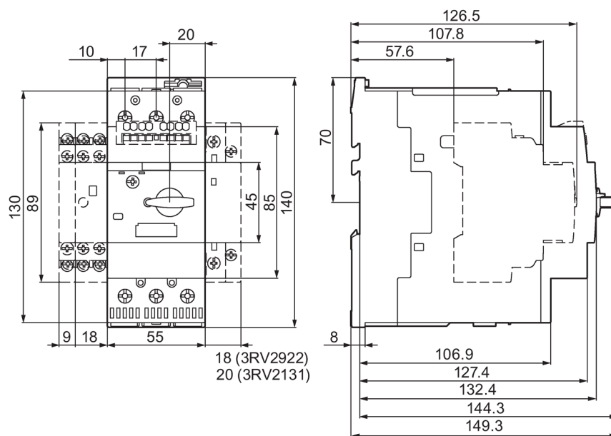
Figure C-11 3RV2.31 ( \geq 52 A) / 3RV2.32 / 3RV2431-4VA1 motor starter protectors.
