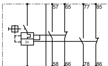
Signaling switch 3RV2921-.M
