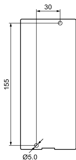
Figure C-15 3RV2.4 motor starter protectors
