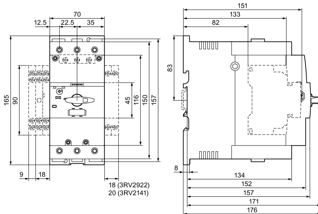
Figure C-13 3RV2.4 motor starter protectors
