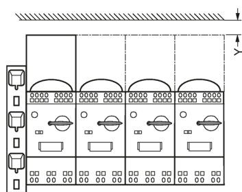
Figure 11-10 Installation guidelines
