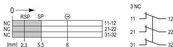
Figure 4-14 3SE2243-6XX
