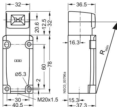
Minimum actuation radius without tumbler
