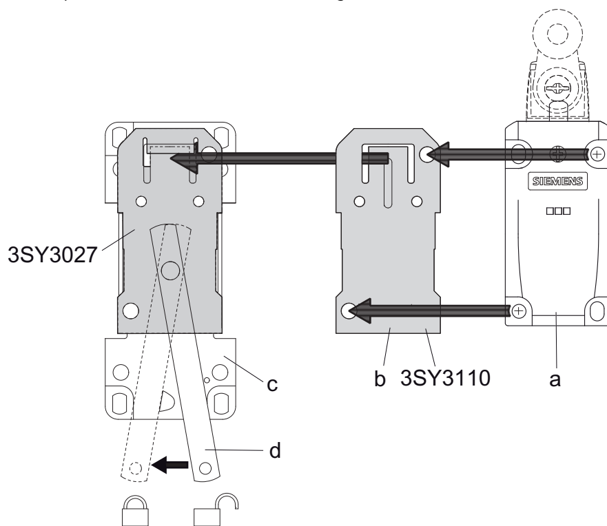
Figure 8-1 Quick-release device
