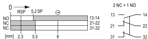
Figure 4-13 3SE2243-0XX
