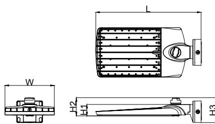
Wall Bracket with Surface Conduit (WBA)
