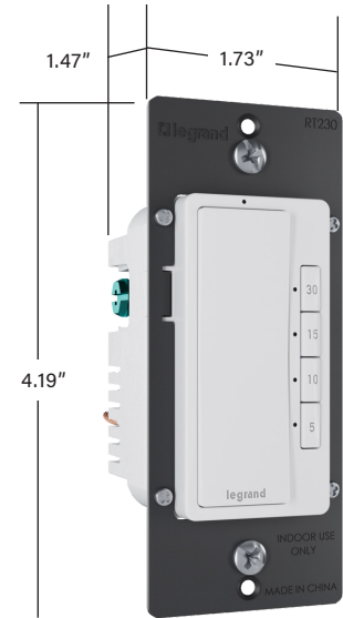
RT230W Depth (Into Wallbox) = 1.19"
