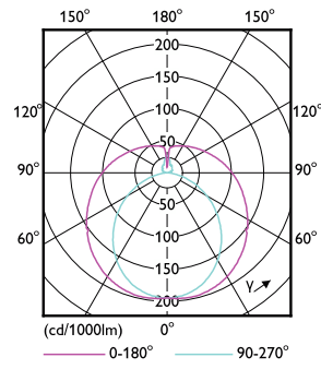
Light Distribution Diagram - 8.4T8/MAS/48-840/MF16/G/DIM UE 25/1
