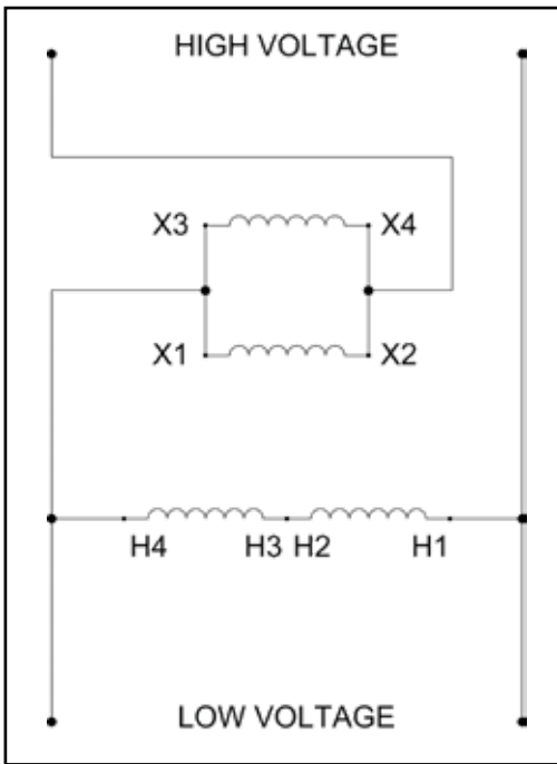
Connection Diagram #3
