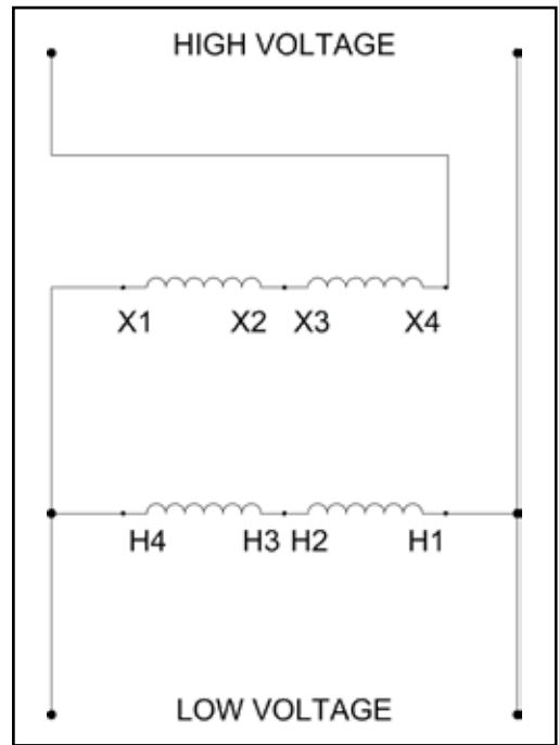
Connection Diagram #4
