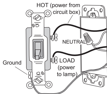
Fig 2: Typical Single Pole Switch Wiring
