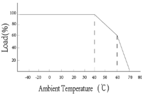
Load vs Ambient Temp Curve
