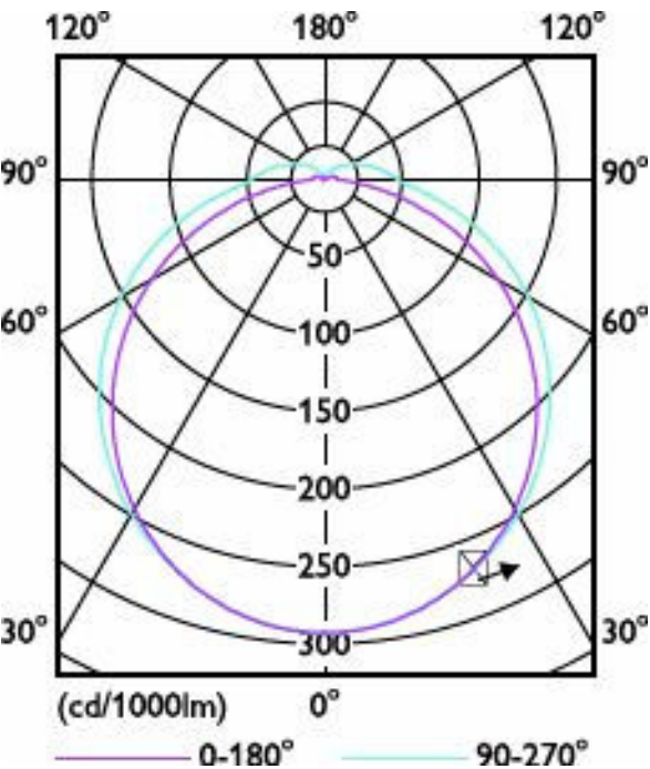
Light Distribution Diagram - SPL-S/LED/13H/827/IF5/P/2P 20/1
