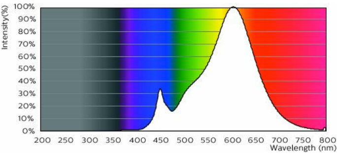
Spectral Power Distribution Colour - SPL-S/LED/13H/827/IF5/P/2P 20/1
