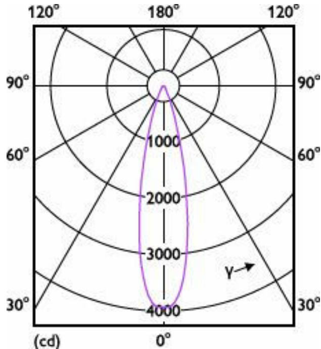
Light Distribution Diagram - 8.5PAR30L/COR/930/F25/D/P/ULW/T20 6/1FB
