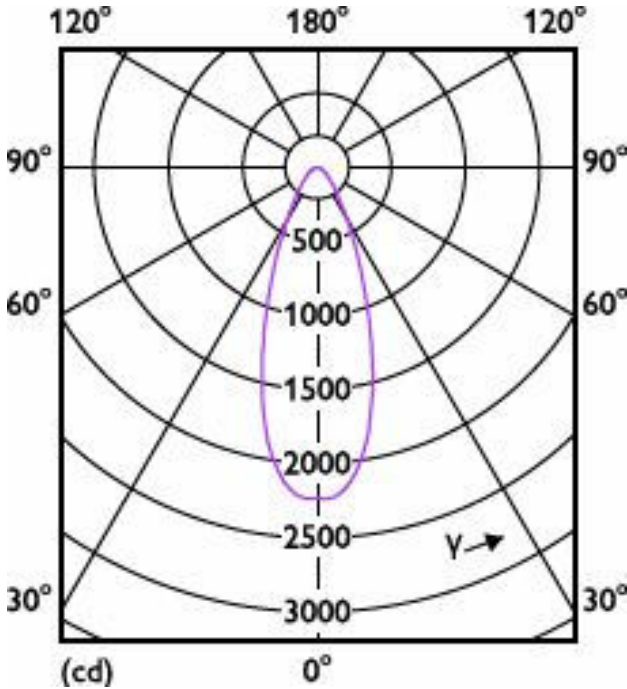
Light Distribution Diagram - 13PAR38/COR/927/F40/DIM/P/ULW/T20 6/1FB
