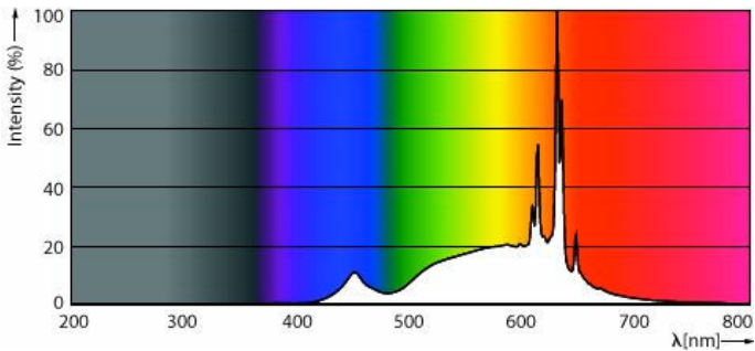
Spectral Power Distribution Colour - 13PAR38/COR/927/F40/DIM/P/ULW/T20 6/1FB
