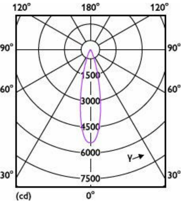
Light Distribution Diagram - 13PAR38/COR/940/F25/DIM/P/ULW/T20 6/1FB
