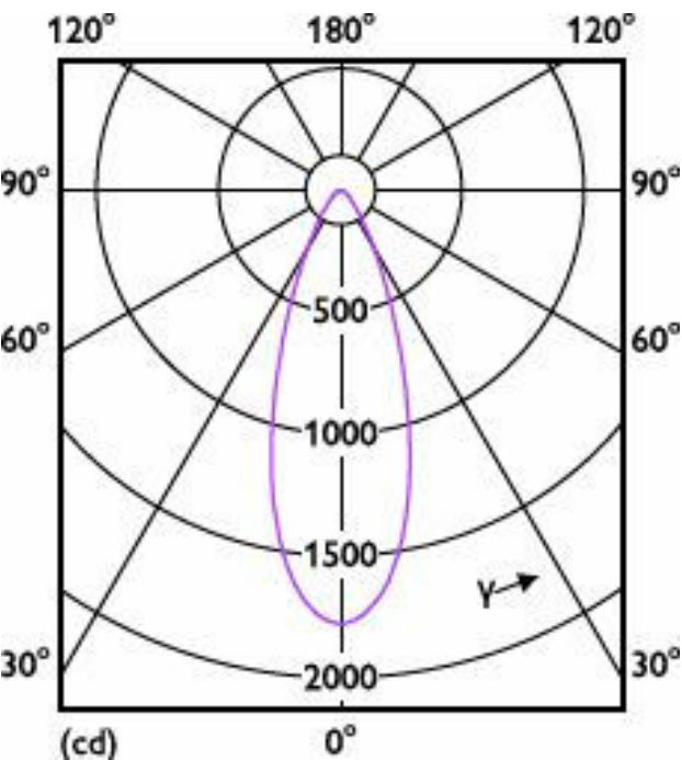
Light Distribution Diagram - 8.5PAR30L/COR/930/F40/D/P/ULW/T20 6/1FB
