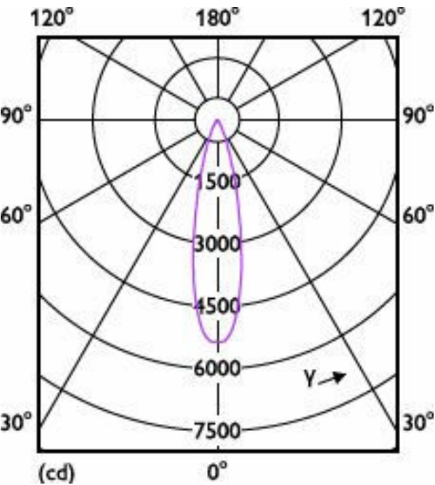
Light Distribution Diagram - 13PAR38/COR/930/F25/DIM/P/ULW/T20 6/1FB
