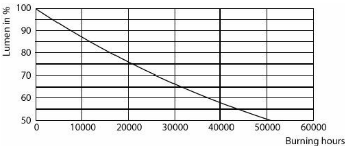
Lumen Maintenance Diagram - 5.5PAR20/COR/ F25/927-922/DIM/P/T20 6/1FB
