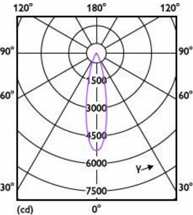
Light Distribution Diagram - 13PAR38/COR/940/F40/DIM/P/ULW/T20 6/1FB
