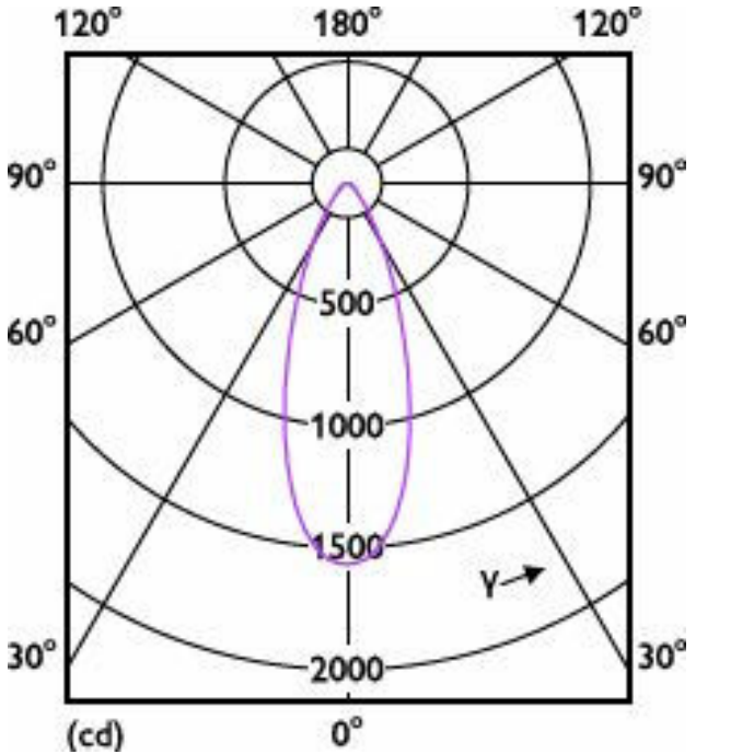
Light Distribution Diagram - 8.5PAR30L/COR/927/F40/D/P/ULW/T20 6/1FB
