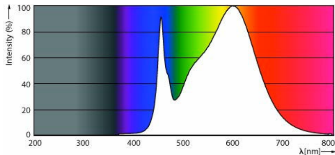
Spectral Power Distribution Colour - 8.4T8/MAS/48-835/ MF16/G/DIM UE 25/1
