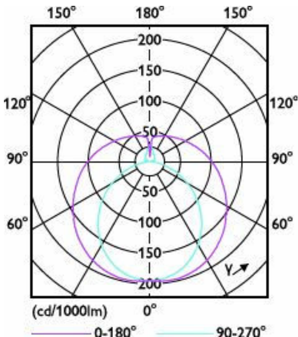
Light Distribution Diagram - 8.4T8/MAS/48-835/MF16/G/DIM UE 25/1
