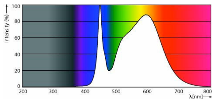
Spectral Power Distribution Colour - 8.4T8/MAS/48-840/ MF16/G/DIM UE 25/1
