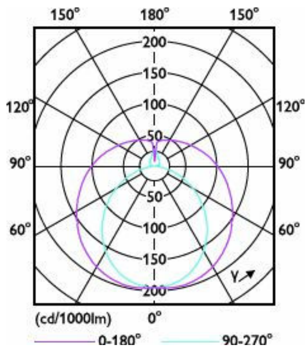
Light Distribution Diagram - 8.4T8/MAS/48-840/MF16/G/DIM UE 25/1
