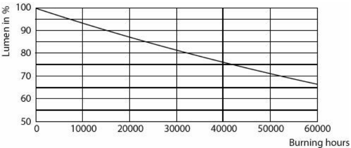
Lumen Maintenance Diagram - 15.3T8/CNG/48-835/MX20/G 25/1
