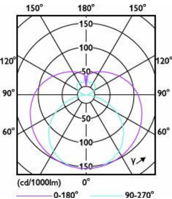
Light Distribution Diagram - 15.3T8/CNG/48-835/MX20/G 25/1
