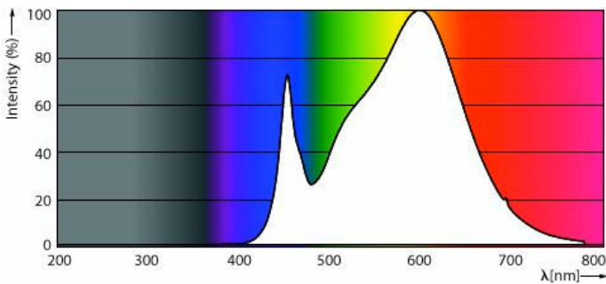
Spectral Power Distribution Colour - 33PAR38/PER/835/F25/DIM/120V 6/1FB
