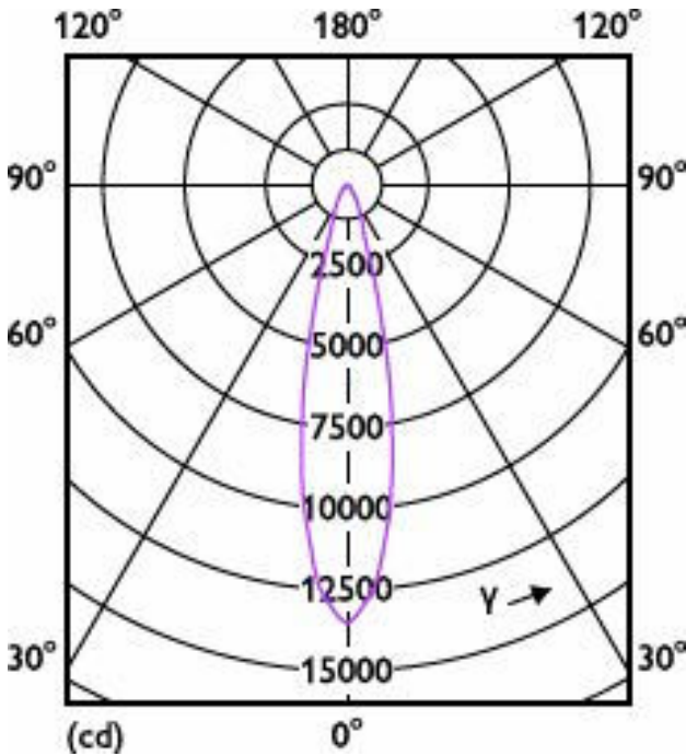
Light Distribution Diagram - 33PAR38/PER/835/F25/DIM/120V 6/1FB
