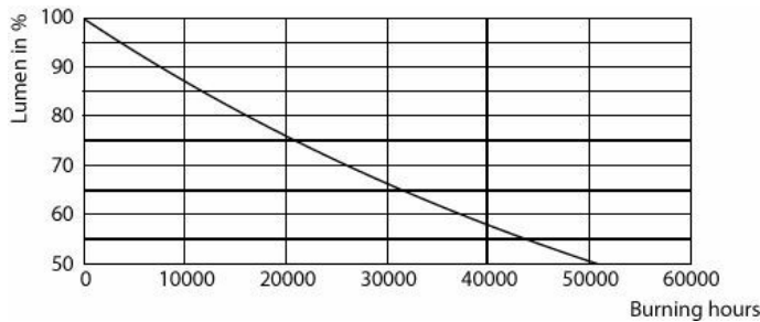
Lumen Maintenance Diagram - 33PAR38/PER/835/F25/DIM/120V 6/1FB
