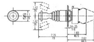
Round Joystick With Interlock
