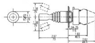
Round Joystick
